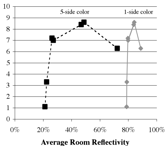
Figure 8: The Average Room Reflectivity (ARR) changes very little within the range of colors from an LRV if only one wall is colored. The ARR changes dramatically when all five sides are colored.
