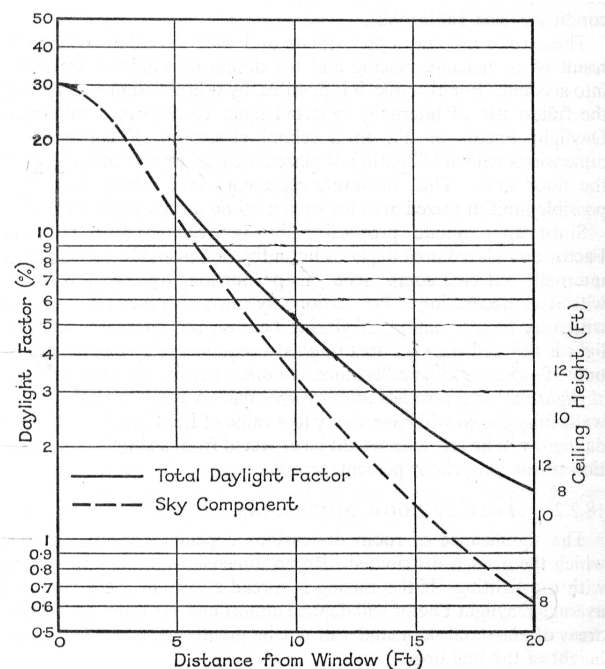
Figure 1: Hopkinson, R.G.: Daylighting. The variation of Sky Component and total Daylight Factor with distance from window for a 8' ceiling height (P. 43).
